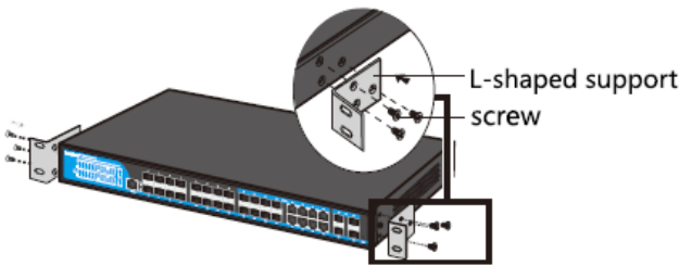
Figure 1.1.1 installation diagram of switch
