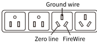
Figure 1.2.1 single phase three wire power socket
