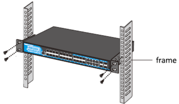
Figure 1.1.2 installation diagram of switch
