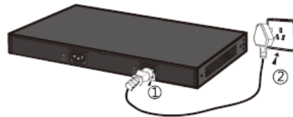
Figure 1.2.2 power connection diagram
