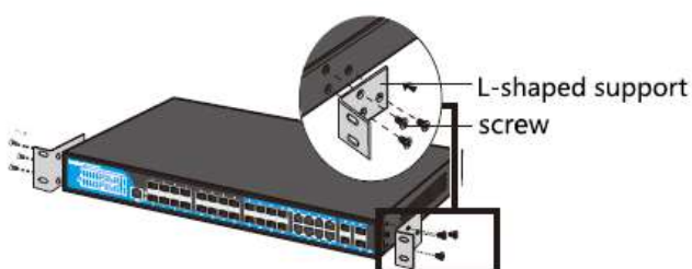
Figure 1.1.1 installation diagram of switch
