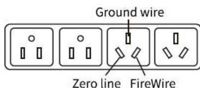
Figure 1.2.1 single phase three wire power socket
